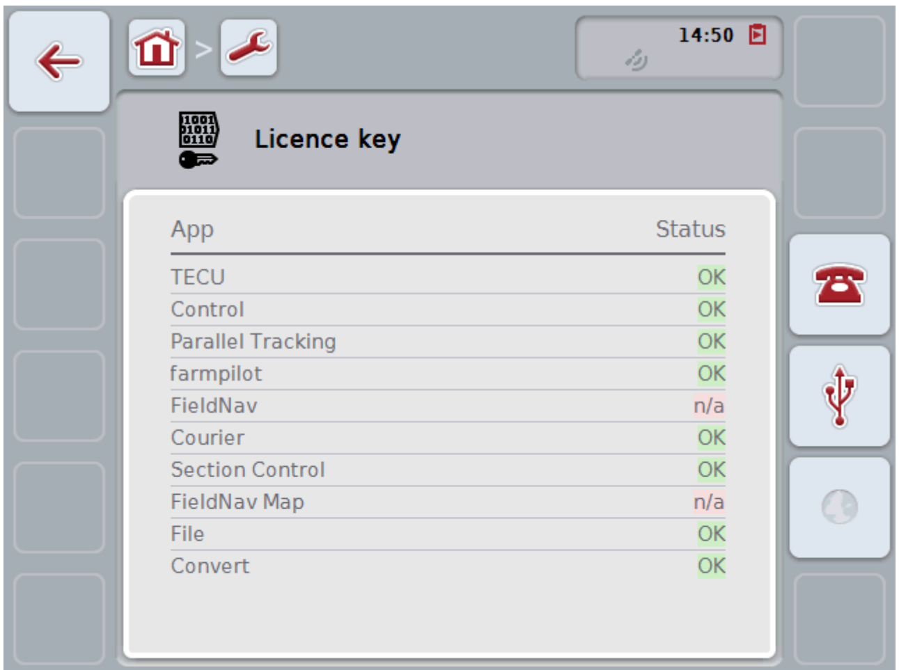
Screen 2. Display activations
